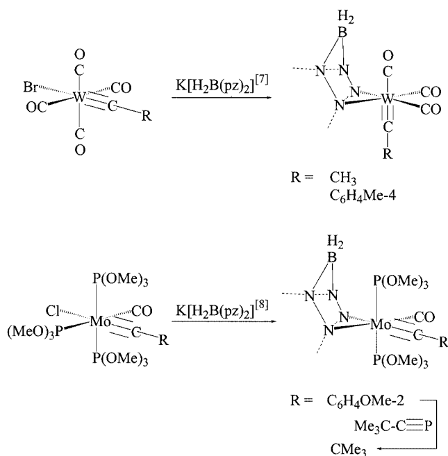
Scheme 2. Dihydrobis(pyrazolyl)borate alkylidyne [7-8]
