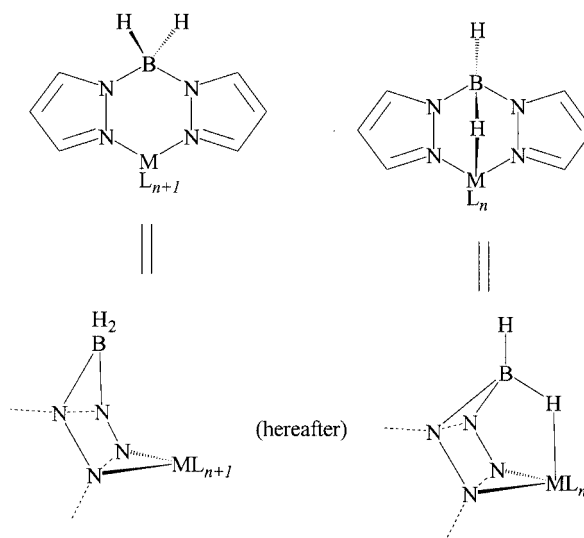
Scheme 1. Dihydrobis(pyrazolyl)borate coordination
